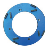
Grinding disc blue HB grit 30/40 Hard bond for soft, abrasive to medium-hard surfaces, e.g. screeds
